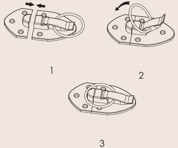
Outer buckle installation method
